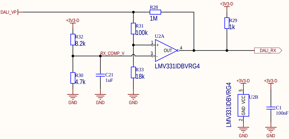
DALI Receiver
