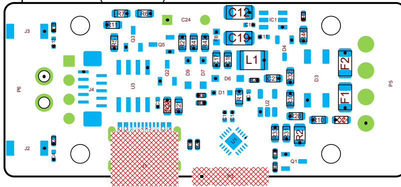
Top SMD/THT (Scale 2:1)
