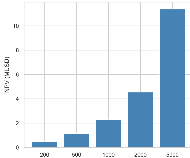
(b) NPV by plant size @100°C
