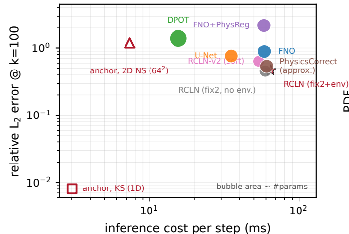
(c) Accuracy-cost Pareto (earlier learned-anchor lineage)
