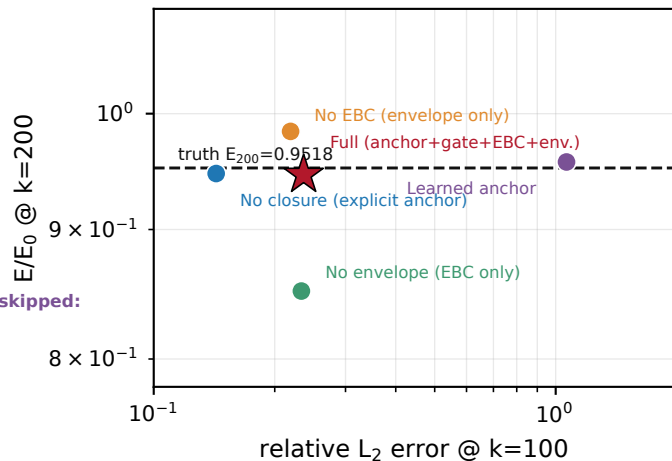
(b) Component ablation (3D TGV, v8)
