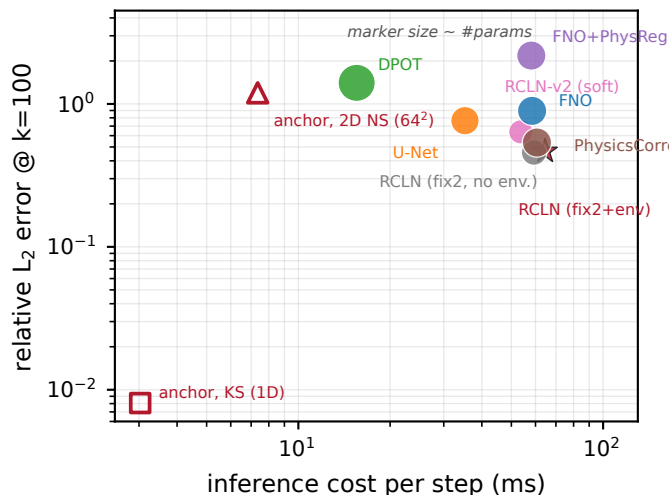
(c) Accuracy-cost Pareto (earlier learned-anchor lineage)
