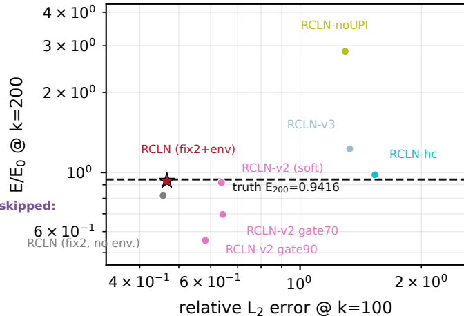
(b) Hard-vs-soft physics ablation (3D TGV)
