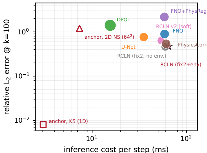
(c) Accuracy-cost Pareto (marker size ~ params)
