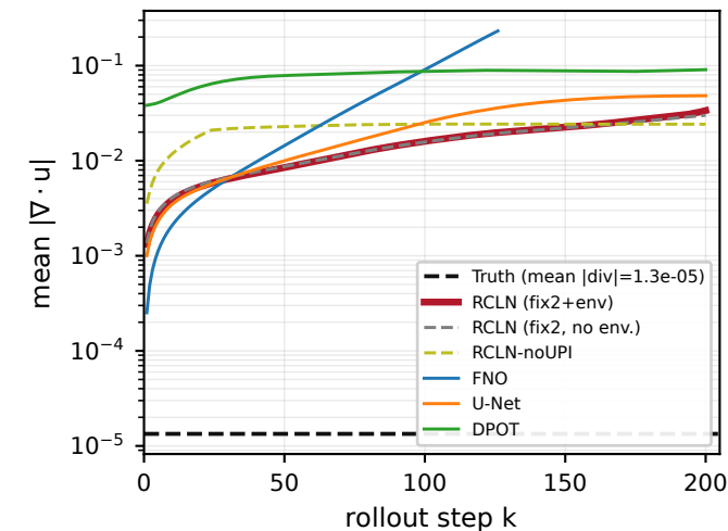
(c) Divergence violation (Thm-1, DNS precision)
