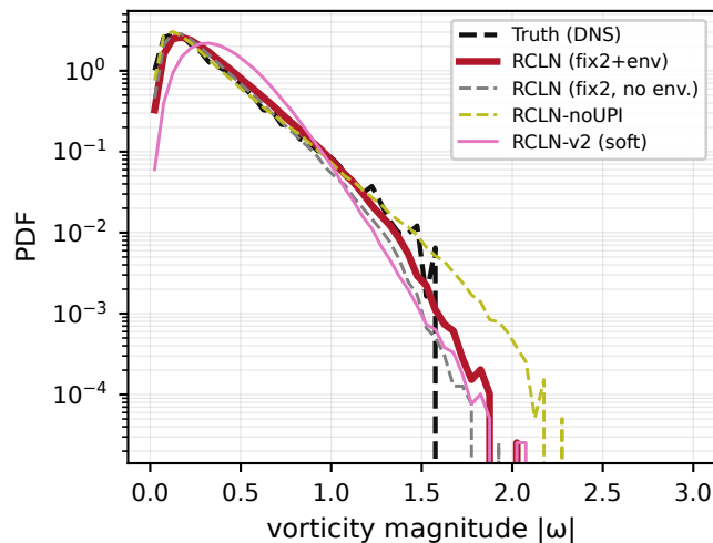
(b) Vorticity PDF at k=200 (3 ICs): tails = vortex cores
