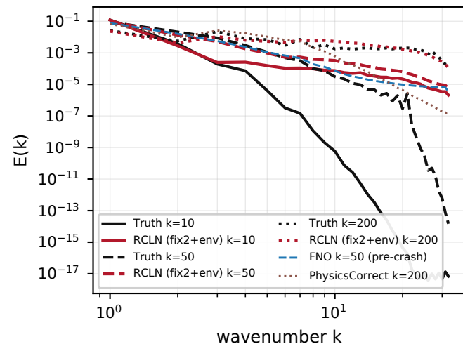
(a) Energy spectrum: high-k behaviour
