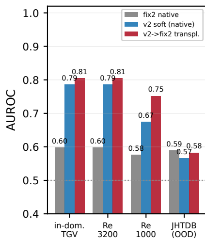
(c) AUROC across distributions
