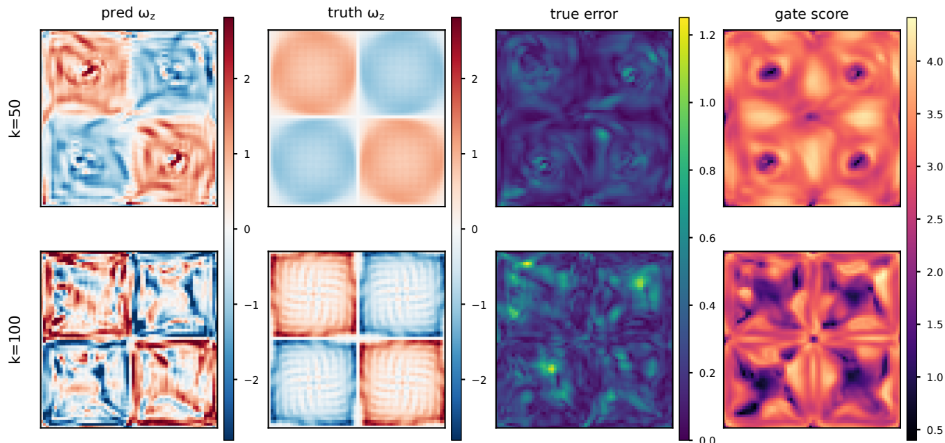
(a) Mid-plane \omega_z : prediction, truth, true error and gate score
