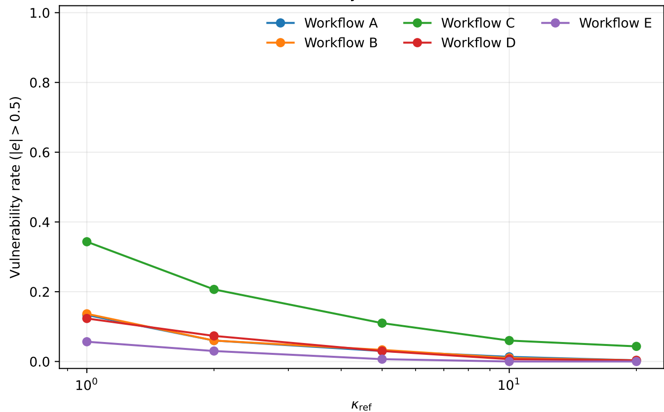
Vulnerability rate ( C=0.6 )
