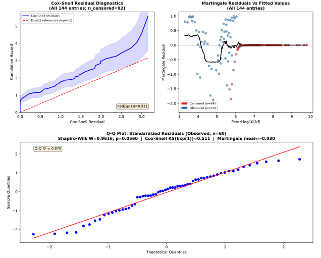
Figure 3: Model diagnostics. Top left: Cox-Snell residual cumulative hazard vs. Exp(1) identity line (all 144 entries). Top right: Martingale residuals vs. fitted \log_{10}(N_f) (all 144 entries; red: censored, blue: observed). Bottom: Q–Q plot of standardized residuals (observed entries, n = 60 ; Shapiro-Wilk W = 0.96 , p = 0.056 , R^2 = 0.97 ).
