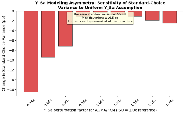
Figure 1: Y_{Sa} baseline sensitivity. The standard-choice variance fraction is plotted against the Y_{Sa} perturbation factor applied to AGMA and FKM entries (ISO entries retain Y_{Sa} = 1.55 ). Within the plausible range ( 0.95 – 1.15\times , shaded), the deviation from baseline (55.3%) is at most -1.1 pp. The ranking (Standard > Roughness > Mean-stress) is preserved throughout.
