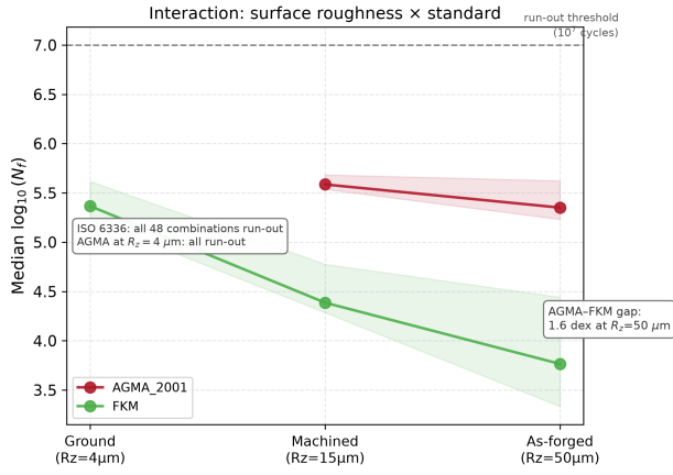
Figure 8: Surface roughness amplifies the divergence between standards: the median AGMA–FKM gap reaches 1.6 dex at R_z = 50\ \mu\text{m} (as-forged). ISO 6336 entries are all run-out (life > 10^7 cycles) at every roughness level, and AGMA entries are likewise all run-out at R_z = 4\ \mu\text{m} (ground), where only FKM retains finite-life predictions. Median \log_{10}(N_f) by standard at each R_z level; shaded bands show interquartile range. All life predictions use the uniform Y_{Sa} = 1.55 baseline.
