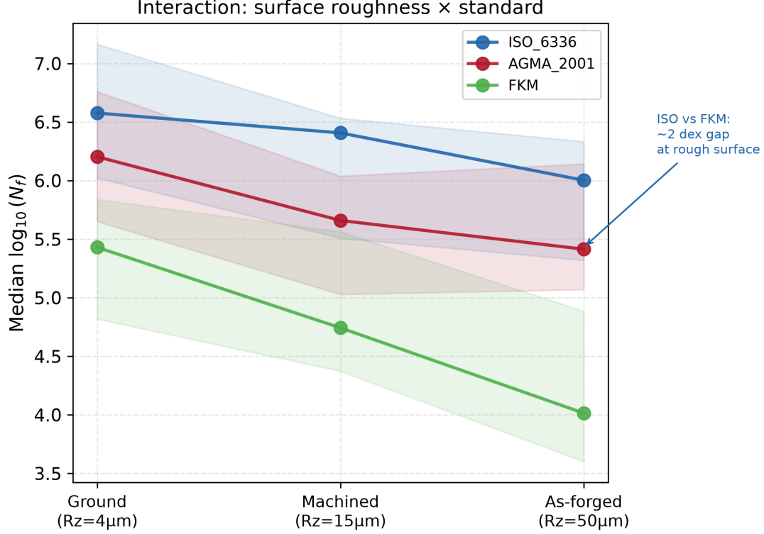
Figure 5: Interaction of surface roughness ( R_z ) and standard. Median \log_{10}(N_f) by standard at each R_z level. Shaded bands show interquartile range.
