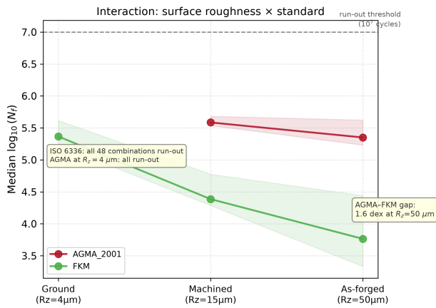
Figure 6: Surface roughness amplifies the divergence between standards: the median AGMA–FKM gap reaches 1.6 dex at R_z = 50 \mu\text{m} (as-forged). ISO 6336 entries are all run-out (life > 10^7 cycles) at every roughness level, and AGMA entries are likewise all run-out at R_z = 4 \mu\text{m} (ground), where only FKM retains finite-life predictions. Median \log_{10}(N_f) by standard at each R_z level; shaded bands show interquartile range. All life predictions use the uniform Y_{Sa} = 1.55 baseline.
