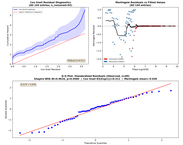
Figure 2: Model diagnostics. Top left: Cox-Snell residual cumulative hazard vs. Exp(1) identity line (all 144 entries). Top right: Martingale residuals vs. fitted \log_{10}(N_f) (all 144 entries; red: censored, blue: observed). Bottom: Q–Q plot of standardized residuals (observed entries, n = 60 ; Shapiro-Wilk W = 0.962 , p = 0.056 , R^2 = 0.970 ).
