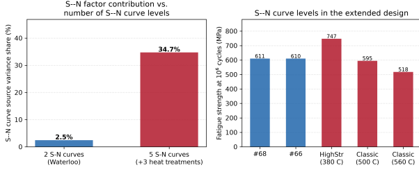
Figure 11: Multi S-N curve sensitivity analysis. Left: S-N source variance share rises from 2.5% (2 nearly-identical Waterloo curves) to 34.7% (5 curves spanning realistic 42CrMo4 heat-treatment states). Right: fatigue strength at 10^6 cycles for the five S-N curve levels. This demonstrates that the baseline 2.5% S-N share is a lower bound reflecting limited material-factor representation, not evidence that material variability is unimportant.
