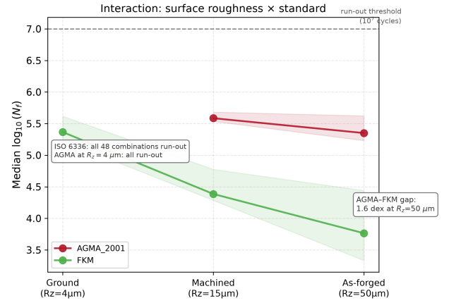
Figure 8: Surface roughness amplifies the divergence between standards: the median AGMA–FKM gap reaches 1.6 dex at R_z = 50 \mu m (as-forged). ISO 6336 entries are all run-out (life > 10^7 cycles) at every roughness level, and AGMA entries are likewise all run-out at R_z = 4 \mu m (ground), where only FKM retains finite-life predictions. Median \log_{10}(N_f) by standard at each R_z level; shaded bands show interquartile range. All life predictions use the uniform Y_{Sa} = 1.55 baseline.
