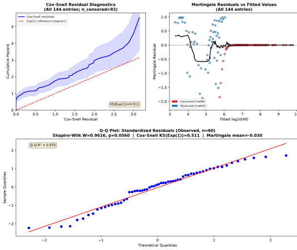
Figure 3: Model diagnostics. Top left: Cox-Snell residual cumulative hazard vs. Exp(1) identity line (all 144 entries). Top right: Martingale residuals vs. fitted \log_{10}(N_f) (all 144 entries; red: censored, blue: observed). Bottom: Q–Q plot of standardized residuals (observed entries, n = 60 ; Shapiro-Wilk W = 0.962 , p = 0.056 , R^2 = 0.970 ).
