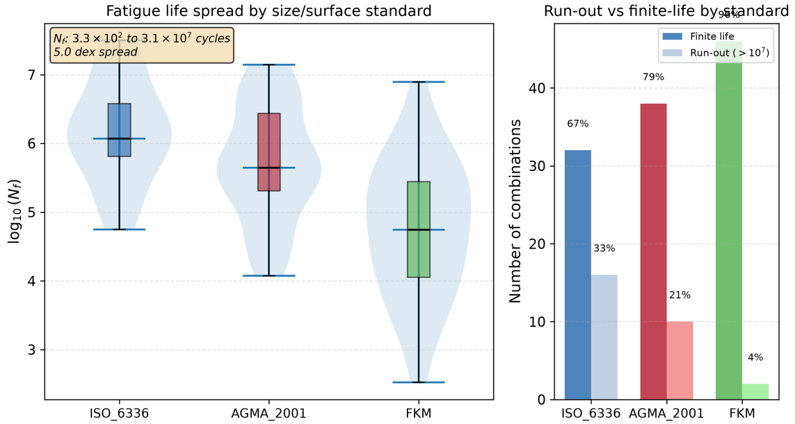
Figure 2: Fatigue life distribution by standard. Left: violin and box plots of \log_{10}(N_f) . Right: run-out vs finite-life counts. N_f spans from 3.3 \times 10^2 to 3.1 \times 10^7 cycles (5.0 dex) among 116 finite-life entries; 28 combinations predict run-out.
