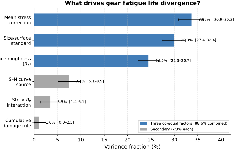
Figure 3: Variance decomposition. Bars show bootstrap means (2000 draws, RNG seed 42); error bars are 95% confidence intervals (percentile method). Point estimates from the single full-model fit are reported in Table 2. Three factors account for 88.6% of total log-variance.
