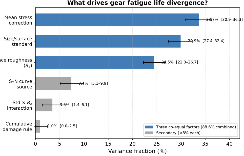
Figure 2: Variance decomposition. Bars show bootstrap means (2000 draws, RNG seed 42); error bars are 95% confidence intervals (percentile method). Point estimates from the single full-model fit are reported in Table 2. Three factors account for 88.6% of total log-variance.
