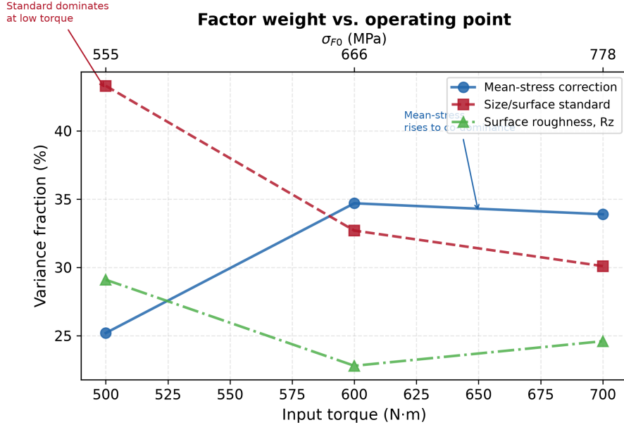
Figure 1: Factor variance shares as a function of input torque (and corresponding nominal tooth-root stress \sigma_{F0} ). At low torque the standard choice dominates; as torque rises toward the endurance limit, mean-stress correction and surface roughness become co-equal with the standard choice. Data from AFT censored-likelihood decomposition at each torque level (Table 3).
