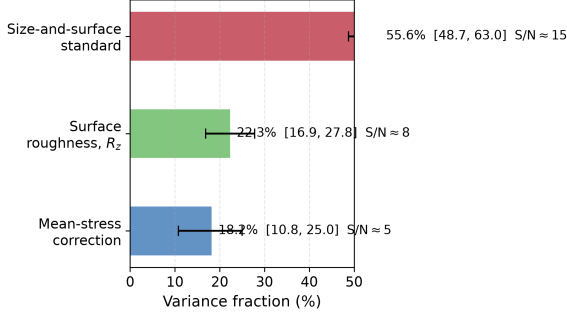
Bootstrap 95% confidence intervals: three dominant factors
