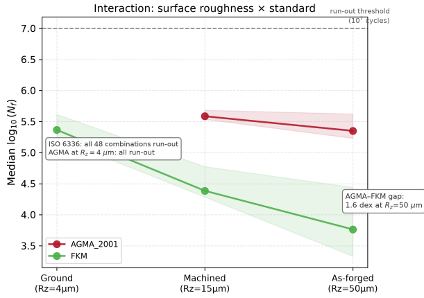
Figure 7: Surface roughness amplifies the divergence between standards: the median AGMA–FKM gap reaches 1.6 dex at R_z = 50 \mu\text{m} (as-forged). ISO 6336 entries are all run-out (life > 10^7 cycles) at every roughness level, and AGMA entries are likewise all run-out at R_z = 4 \mu\text{m} (ground), where only FKM retains finite-life predictions. Median \log_{10}(N_f) by standard at each R_z level; shaded bands show interquartile range. All life predictions use the uniform Y_{Sa} = 1.55 baseline.
