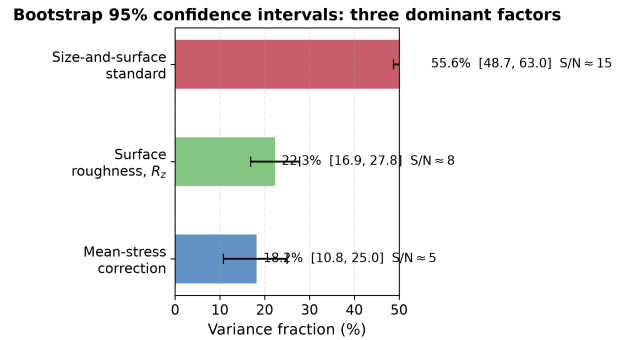
Figure 4: Bootstrap 95% confidence intervals (2000 draws, RNG seed 42) for the three dominant factors. The size-and-surface standard has S/N \approx 15 , confirming that its dominance in Table 2 is robust to resampling and not an artifact of the particular 144-combination dataset. Bars show bootstrap means (standard 55.6% vs. the 55.3% point estimate in Table 2); the small difference reflects resampling variability (§3). Shares are conditional on the common ISO Y_{Sa} baseline and are lower bounds on full standard divergence (§2.3).
