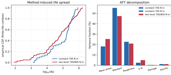
Figure 3: Two-level block-spectrum illustration (supplementary result). Left: empirical CDF of \log_{10}(N_f) across the 144 combinations under constant 700 N·m loading and under a two-level 700/800 N·m block spectrum (1 000 cycles per level per block). Right: AFT drop-one-factor variance fractions under both loadings. The damage-rule share remains \approx 0.3\% under both because the D_c -type formulations are a pure log-scale factor; a larger variable-amplitude damage-rule contribution requires sequence-effect models (Phase 2). @source: output/two_level_variable_amplitude.json
