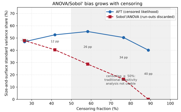
Figure 9: ANOVA/Sobol’ bias versus censoring fraction (supplementary result). The size-and-surface standard share is shown for the AFT censored-likelihood decomposition and for Sobol’/ANOVA (run-outs discarded) across five torque levels (600–800 N·m, censoring 26–89%). The gap grows from \approx 0 pp at 26% censoring to 40 pp at 89%, reproducing the 26.5 pp under-recovery of Table 4 at the reference 58%. @source: output/sobol_censoring_gradient.json
