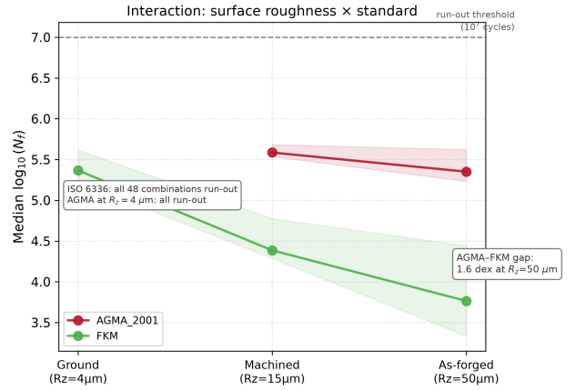
Figure 7: Surface roughness amplifies the divergence between standards: the median AGMA–FKM gap reaches 1.6 dex at R_z = 50\ \mu\text{m} (as-forged). ISO 6336 entries are all run-out (life > 10^7 cycles) at every roughness level, and AGMA entries are likewise all run-out at R_z = 4\ \mu\text{m} (ground), where only FKM retains finite-life predictions. Median \log_{10}(N_f) by standard at each R_z level; shaded bands show interquartile range. All life predictions use the uniform Y_{Sa} = 1.55 baseline.
