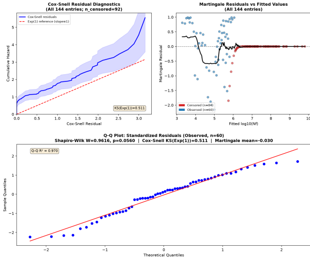
Figure 2: Model diagnostics. Top left: Cox-Snell residual cumulative hazard vs. Exp(1) identity line (all 144 entries). Top right: Martingale residuals vs. fitted \log_{10}(N_f) (all 144 entries; red: censored, blue: observed). Bottom: Q-Q plot of standardized residuals (observed entries, n = 60 ; Shapiro-Wilk W = 0.962 , p = 0.056 , R^2 = 0.970 ).
