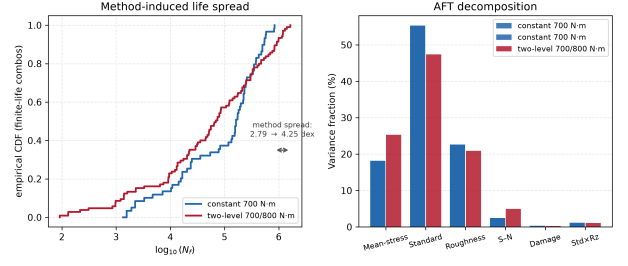
Figure 3: Two-level block-spectrum illustration (supplementary result). Left: empirical CDF of \log_{10}(N_f) across the 144 combinations under constant 700 N·m loading and under a two-level 700/800 N·m block spectrum (1000 cycles per level per block). Right: AFT drop-one-factor variance fractions under both loadings. The damage-rule share remains \approx 0.3\% under both because the D_c -type formulations are a pure log-scale factor; a larger variable-amplitude damage-rule contribution requires sequence-effect models (Phase 2). @source: output/two_level_variable_amplitude.json
