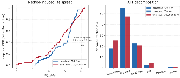
Figure 4: Two-level block-spectrum illustration (supplementary result). Left: empirical CDF of \log_{10}(N_f) across the 144 combinations under constant 700 N·m loading and under a two-level 700/800 N·m block spectrum (1000 cycles per level per block). Right: AFT drop-one-factor variance fractions under both loadings. The damage-rule share remains \approx 0.3\% under both because the D_c -type formulations are a pure log-scale factor; a larger variable-amplitude damage-rule contribution requires sequence-effect models (Phase 2).
