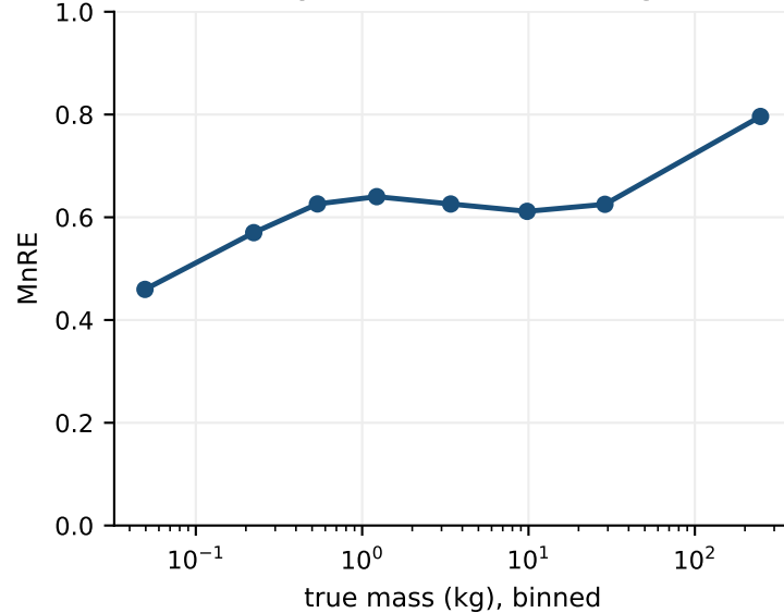
(c) Accuracy across the mass range
