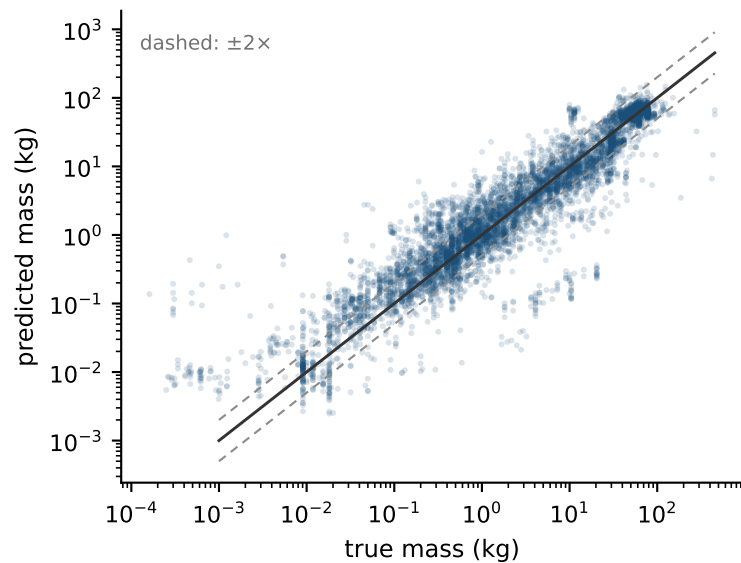
(a) Predicted vs true 70% within 2×
