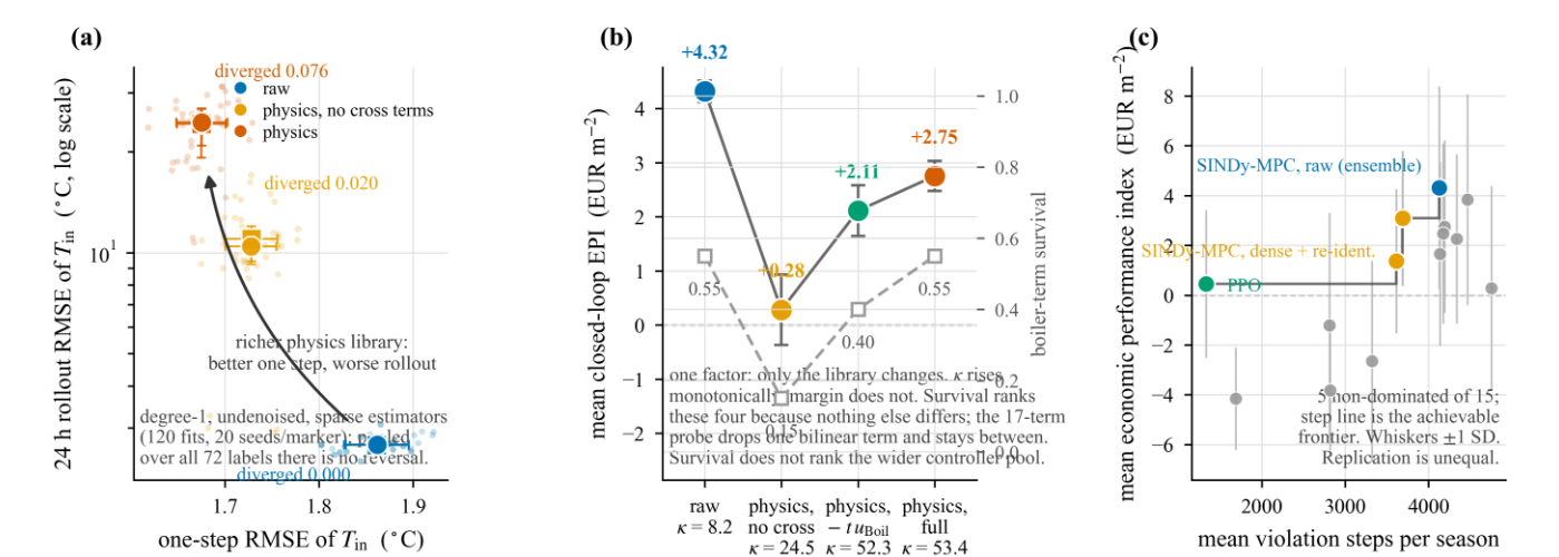
Graphical Abstract. (a) The selection reversal in the first-order, undenoised block under sparse estimators: candidate libraries ordered by one-step prediction error are ordered inversely by 24 h rollout error and by divergence rate. (b) Changing only the feature library, the condition number and the open-loop rollout error rise monotonically across the nested libraries while closed-loop margin does not — the worst-conditioned library outperforms the intermediate one, and the 17-feature probe that deletes the single bilinear boiler term stays at the full library’s level, rejecting the bypass explanation — and the margin instead follows the fraction of fits in which the direct boiler coefficient survives thresholding. (c) The two-axis outcome over four test seasons under the priced objective: the front holds five of the fifteen controllers, so the economic advantage of the raw library is not Pareto-dominant. Sources are named in the LaTeX comment preceding this caption.
