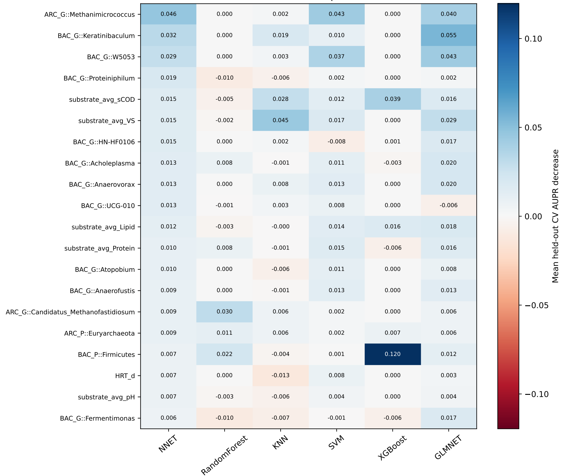
warning_ammonia_toxicity CV AUPR decrease · NNET top 20 across models
