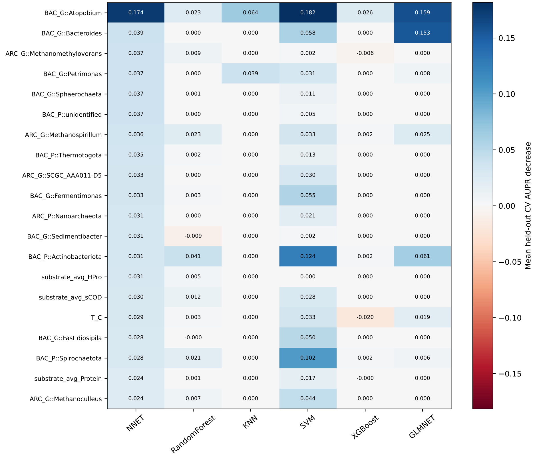
warning_biogas_quality CV AUPR decrease · NNET top 20 across models
