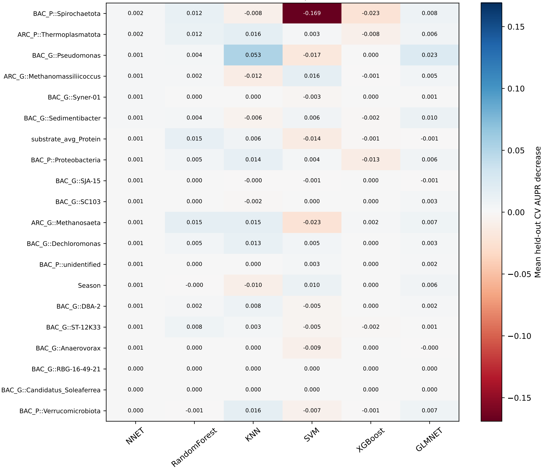
warning_buffer_capacity CV AUPR decrease · NNET top 20 across models
