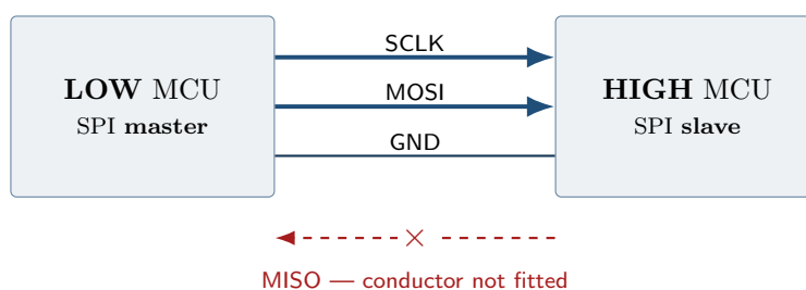
Figure 5: A three-wire SPI diode. Every conductor is driven by the SOURCE side and read by the DESTINATION side; the return data line is not fitted.
