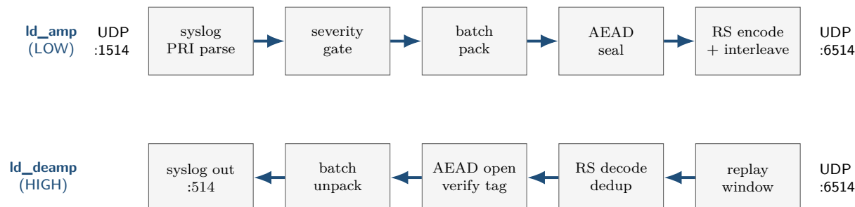
Figure 6: Sender and receiver pipelines. Sealing happens before erasure coding, so the code protects ciphertext and a decode failure and a forgery are the same event to the receiver: a tag that does not verify.
