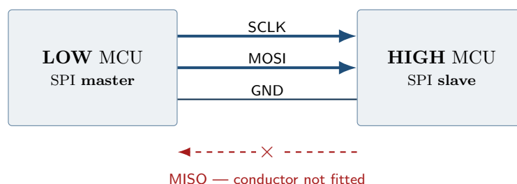
Figure 5: A three-wire SPI diode. Every conductor is driven by the LOW side and read by the HIGH side; the return data line is not fitted.
