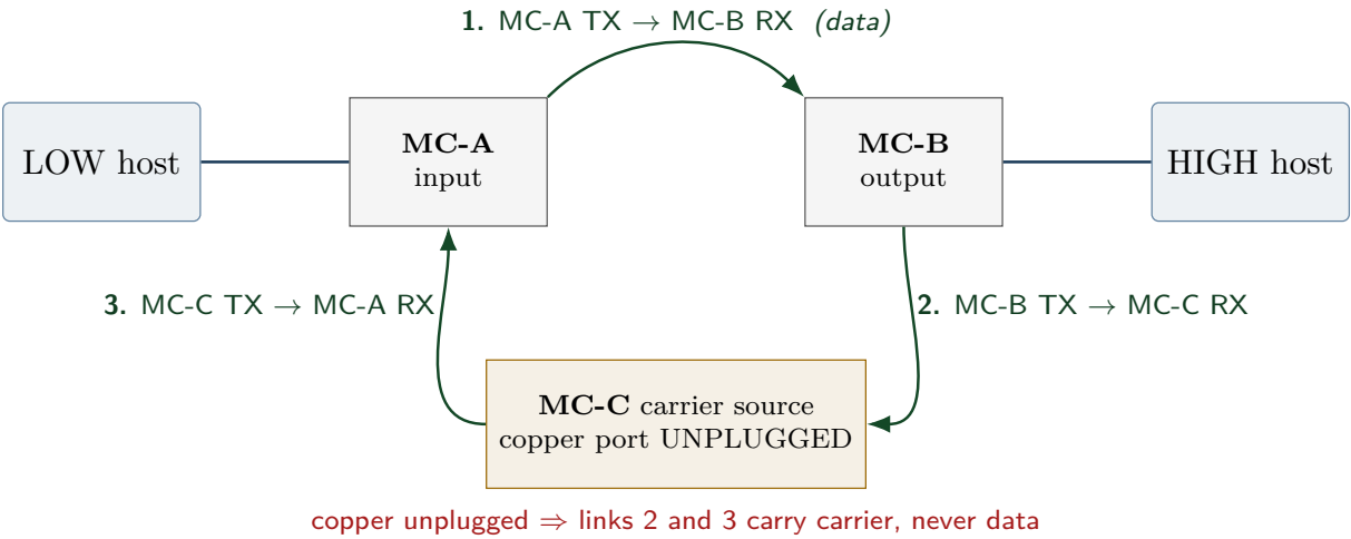
Figure 4: Three-converter diode. The security argument rests on one unplugged copper port.
