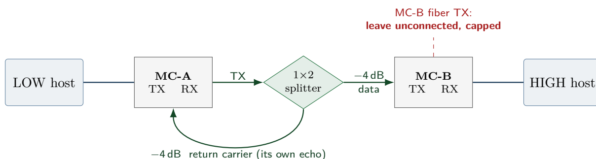
Figure 3: Two-converter diode. The splitter is passive and reciprocal, so the unused legs matter as much as the used ones.
