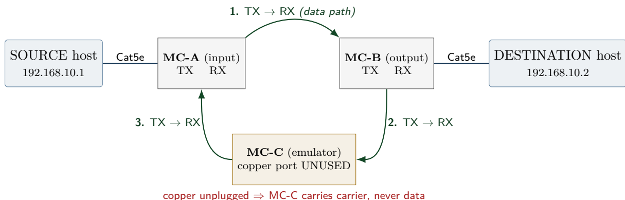
Figure 2: Three-converter diode. Data travels only along link 1. Links 2 and 3 exist solely so MC-A sees carrier on its RX port; because MC-C’s copper port is unplugged, no data can traverse them.
