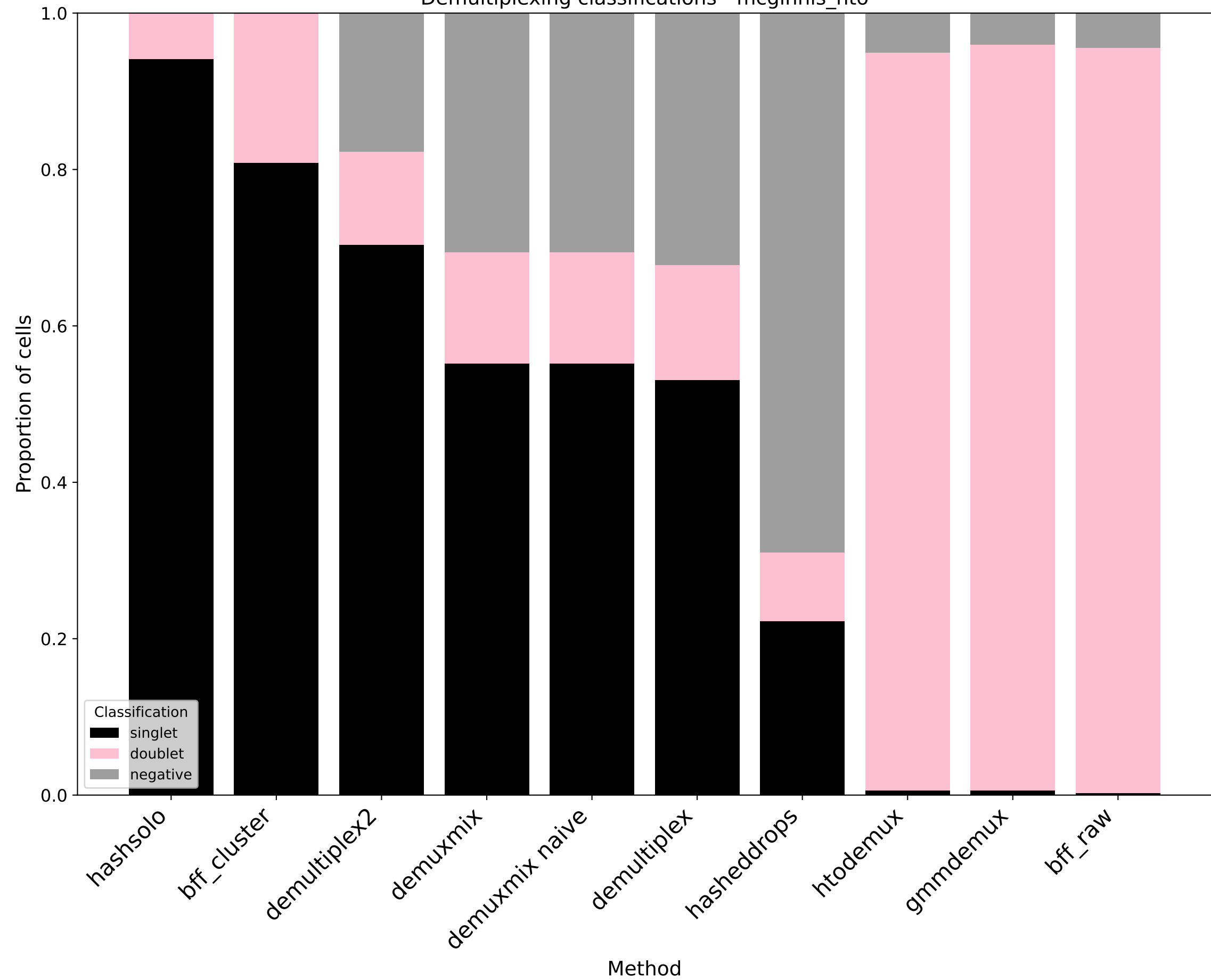
Demultiplexing classifications - mcginnis_hto
