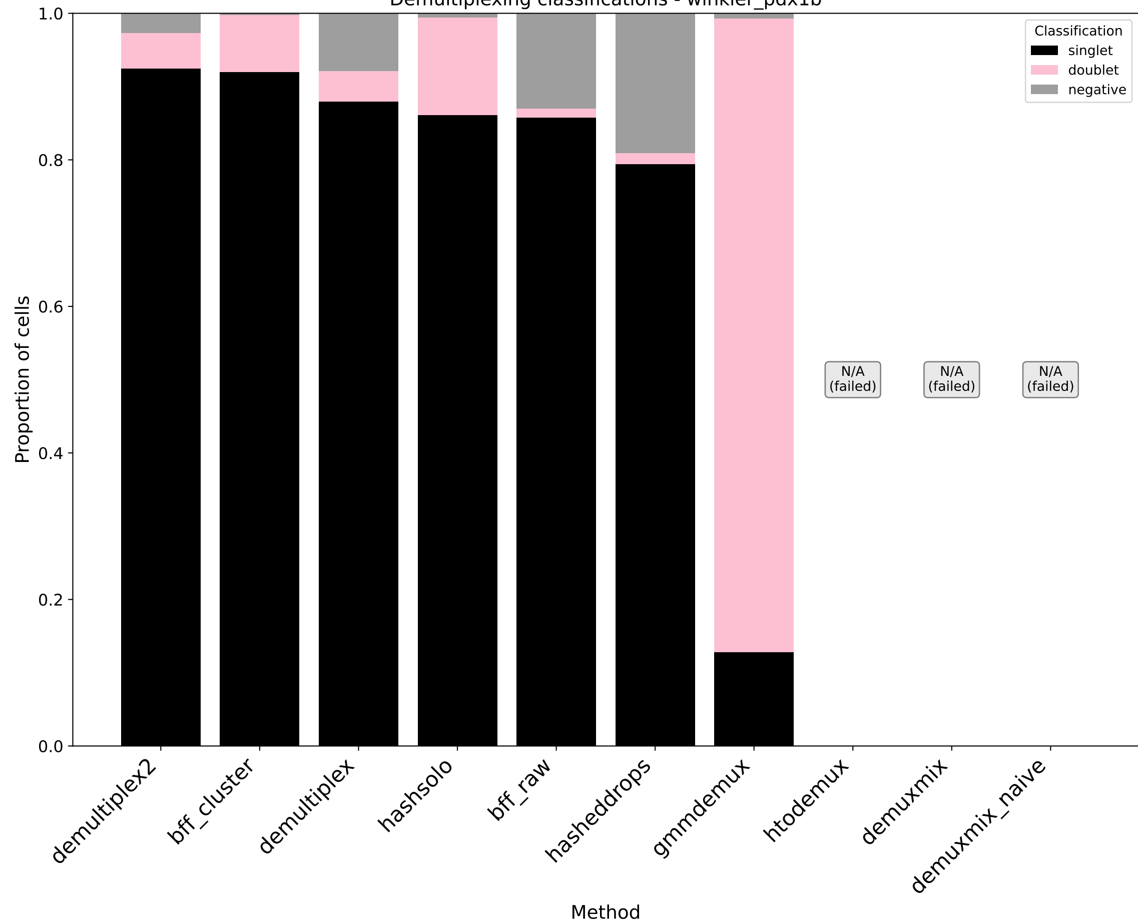
Demultiplexing classifications - winkler_pdx1b
