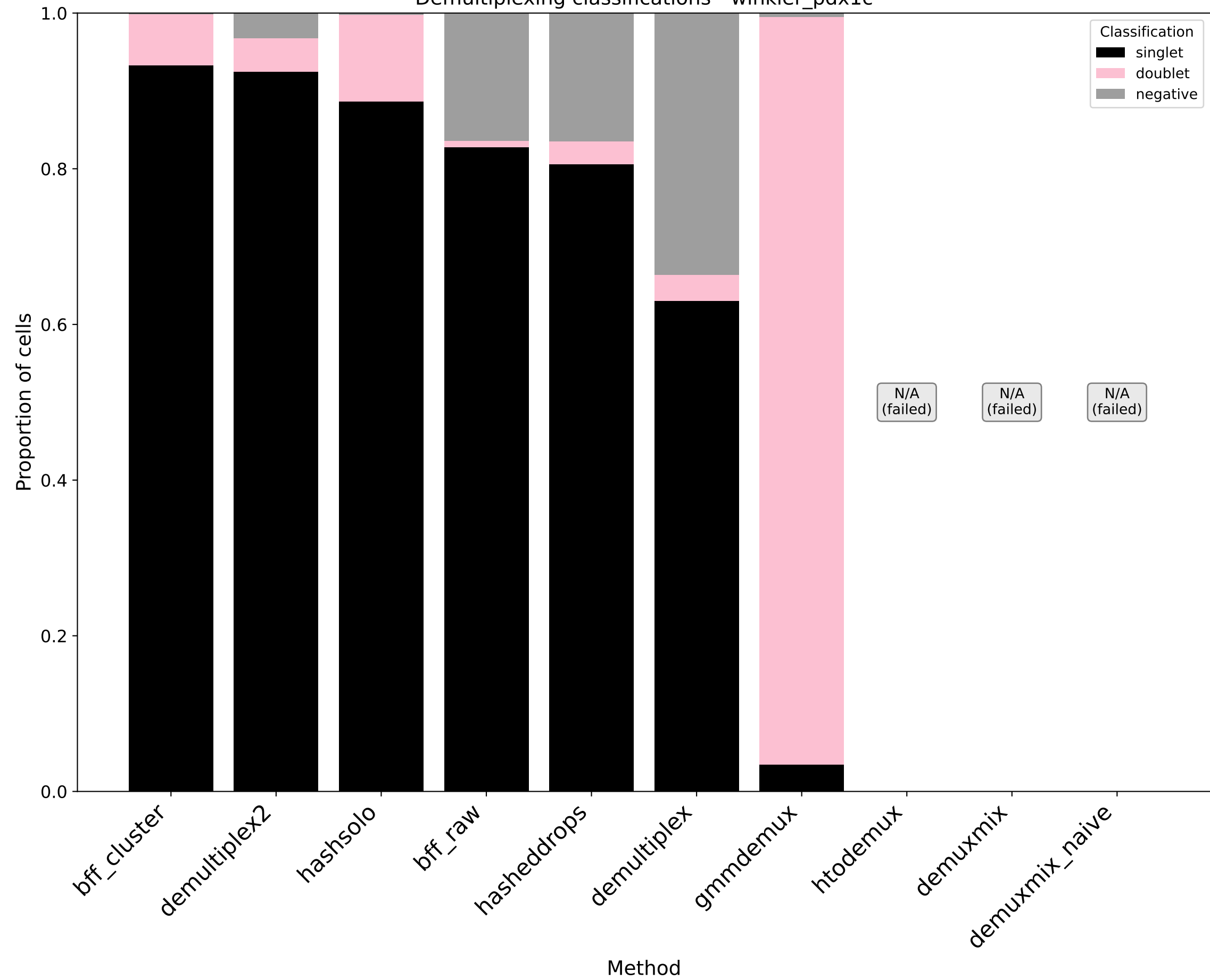
Demultiplexing classifications - winkler_pdx1c
