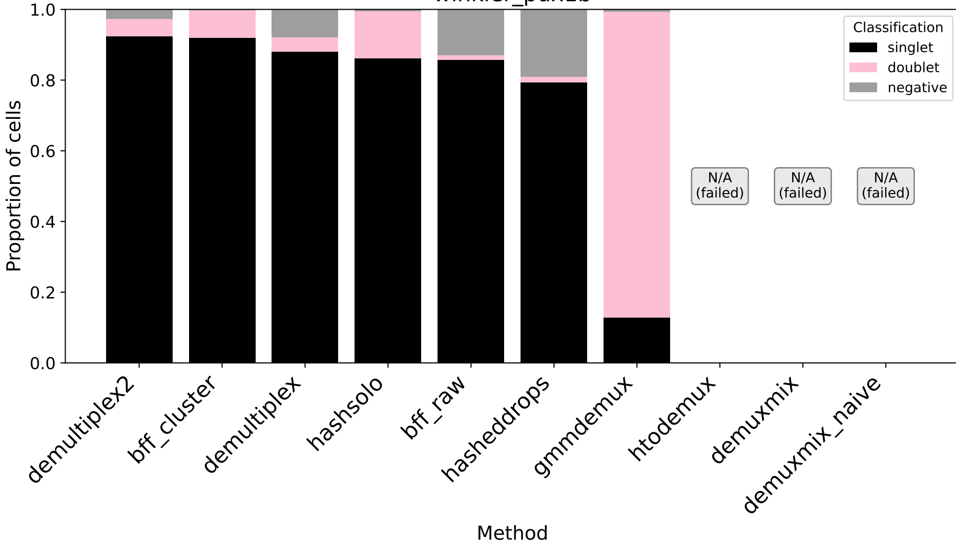
winkler_pdx1b
