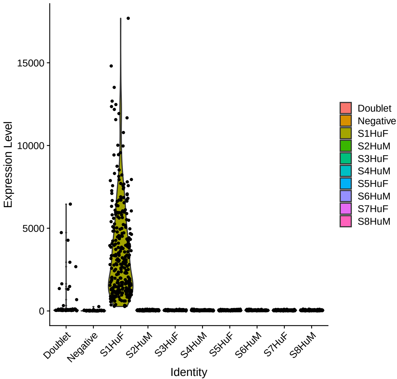
bff_cluster: S1HuF
