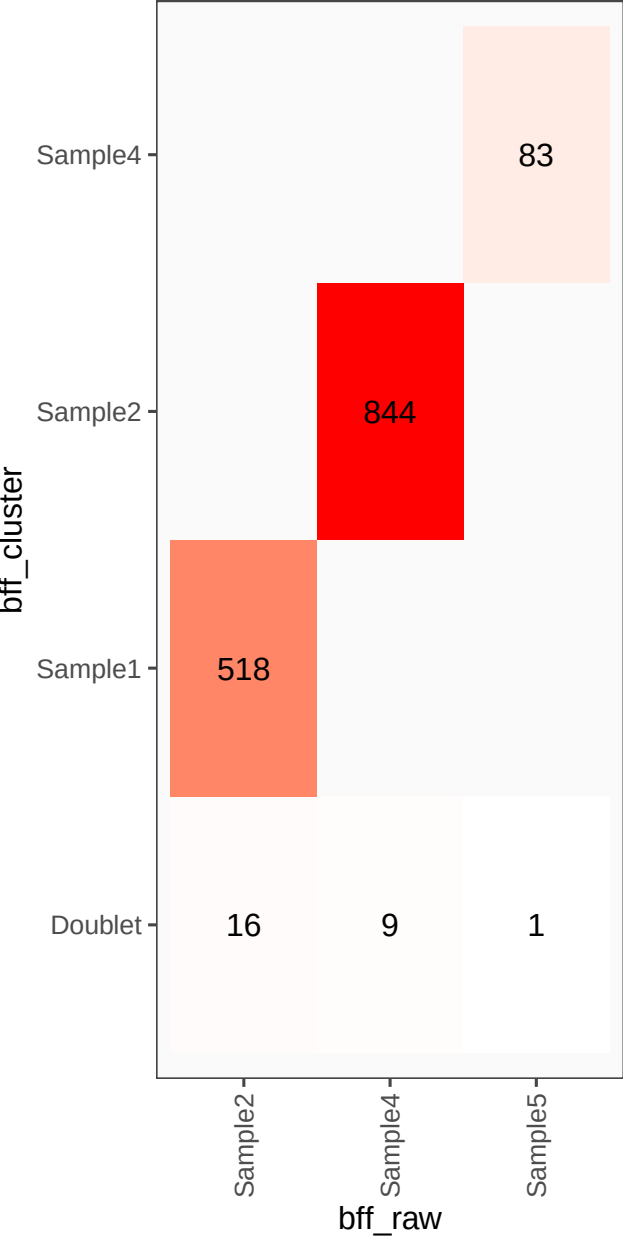
Discordant calls: bff_raw vs. bff_cluster
