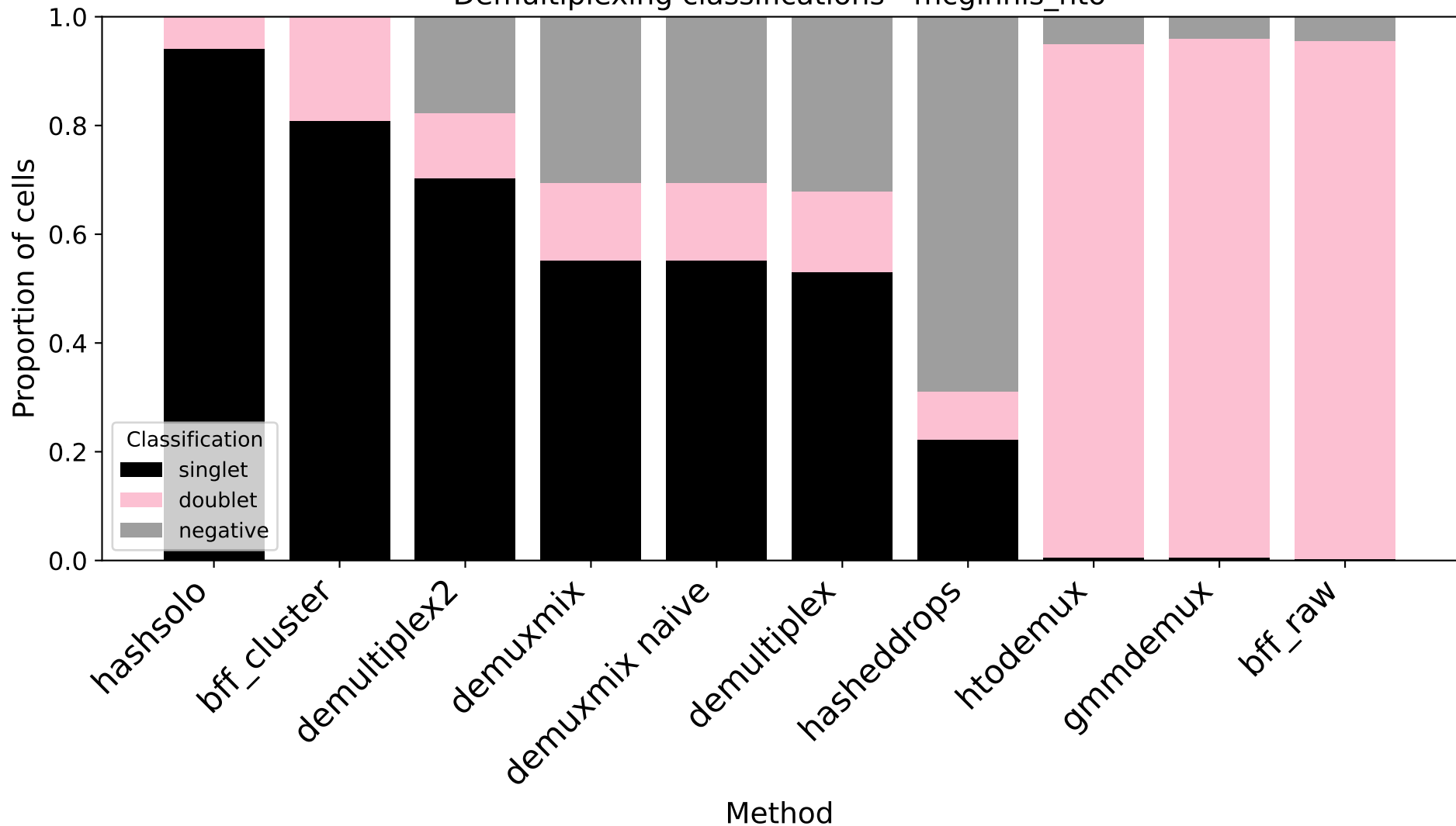
Demultiplexing classifications - mcginnis_hto
