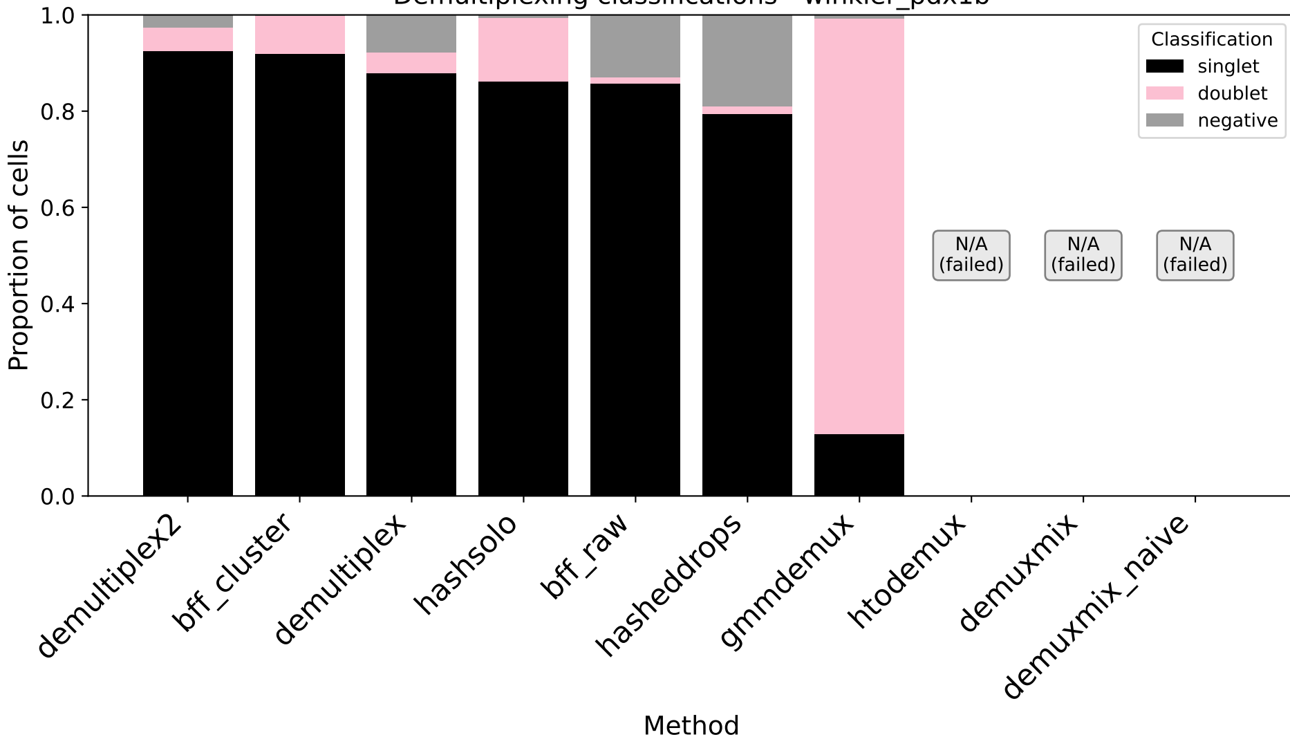
Demultiplexing classifications - winkler_pdx1b
