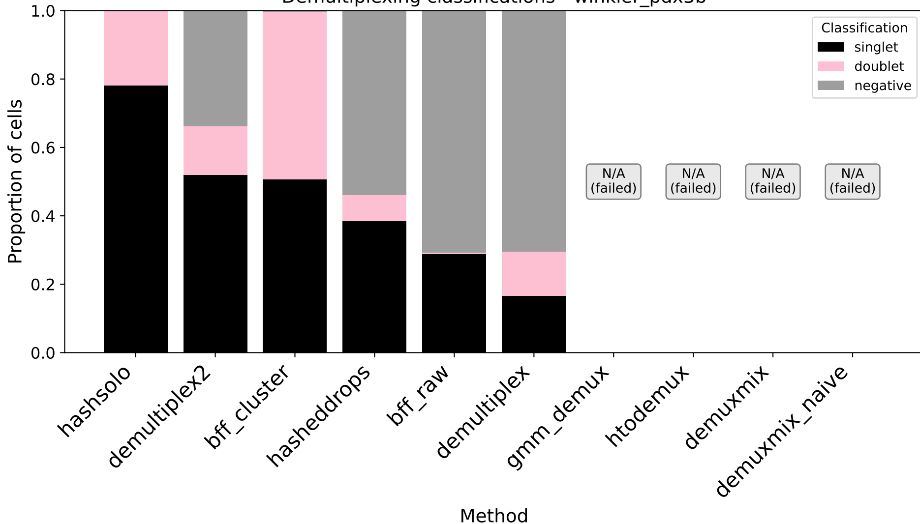
Demultiplexing classifications - winkler_pdx3b
