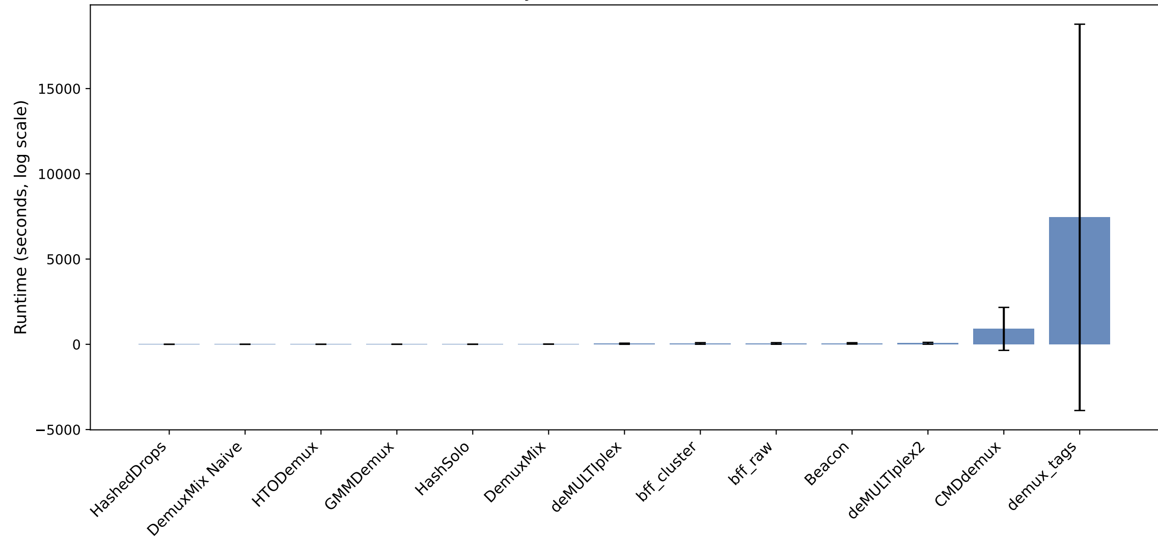
Mean Runtime by Method ( \pm std dev across datasets)
