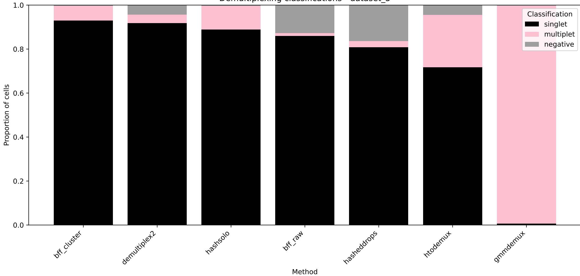
Demultiplexing classifications - dataset_5
