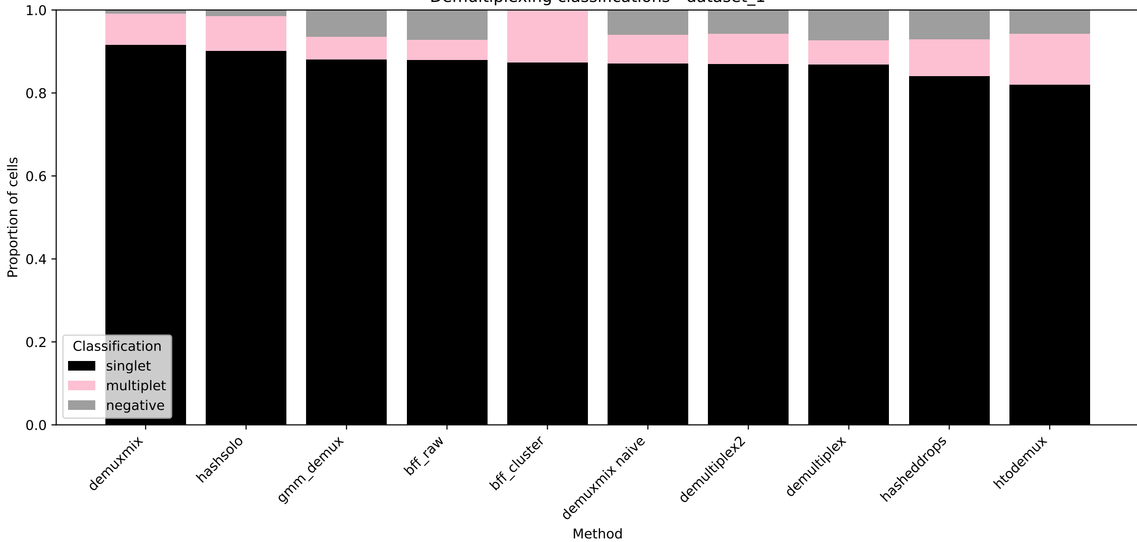
Demultiplexing classifications - dataset_1
