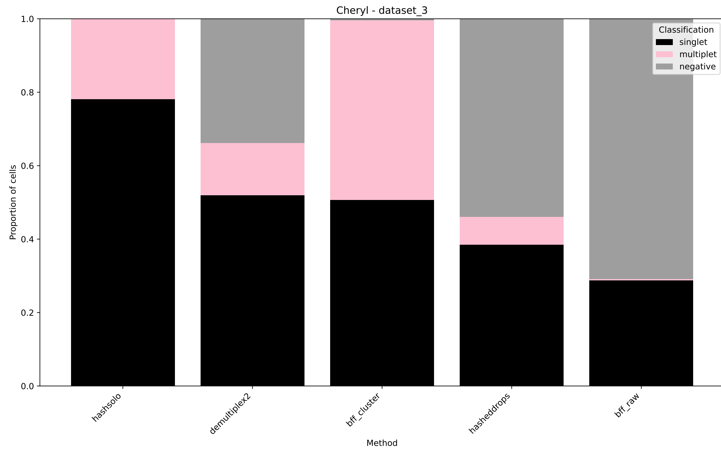
Demultiplexing classifications - dataset_3
