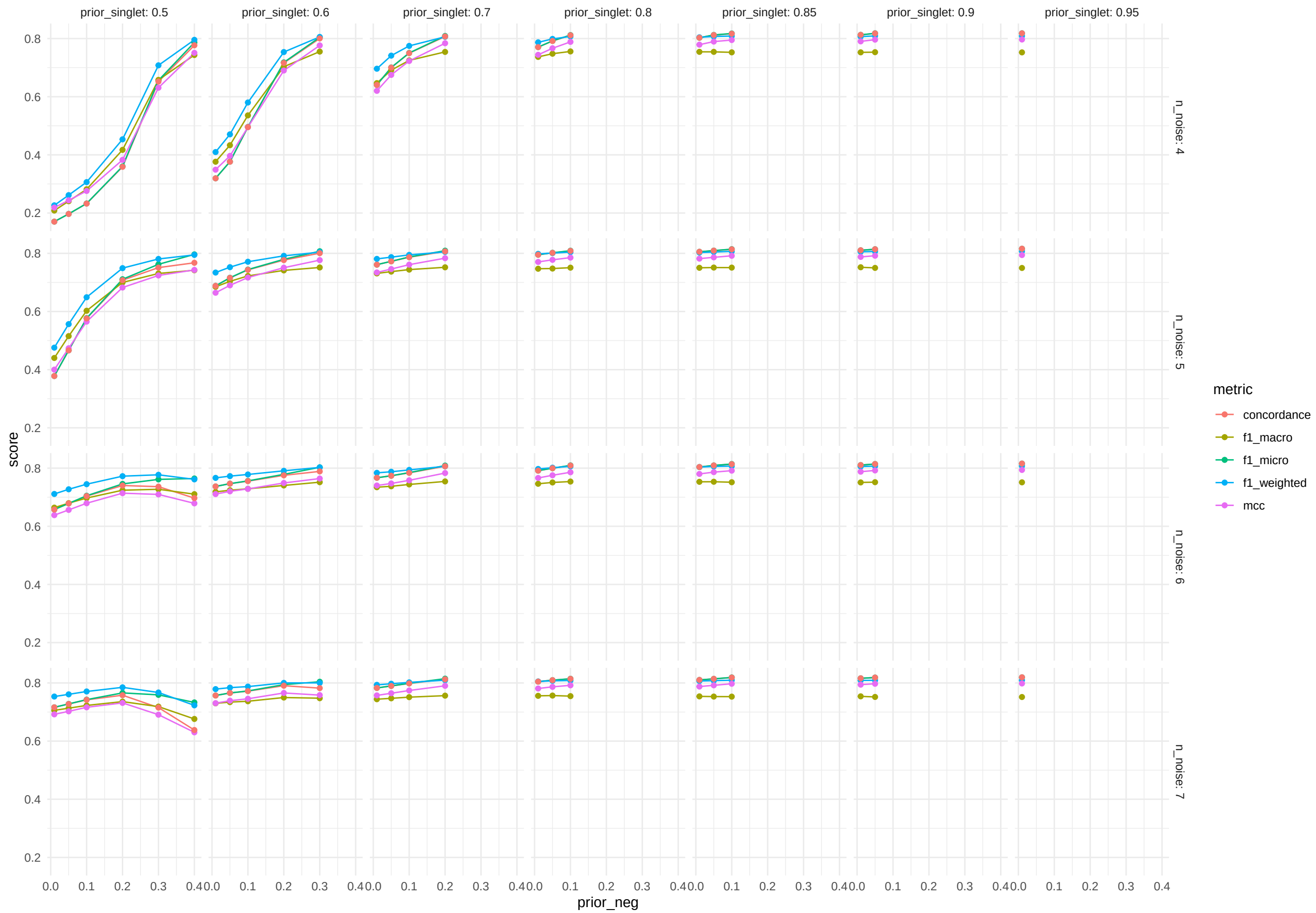
HashSolo – all metrics vs prior_neg – mcginnis_ab
