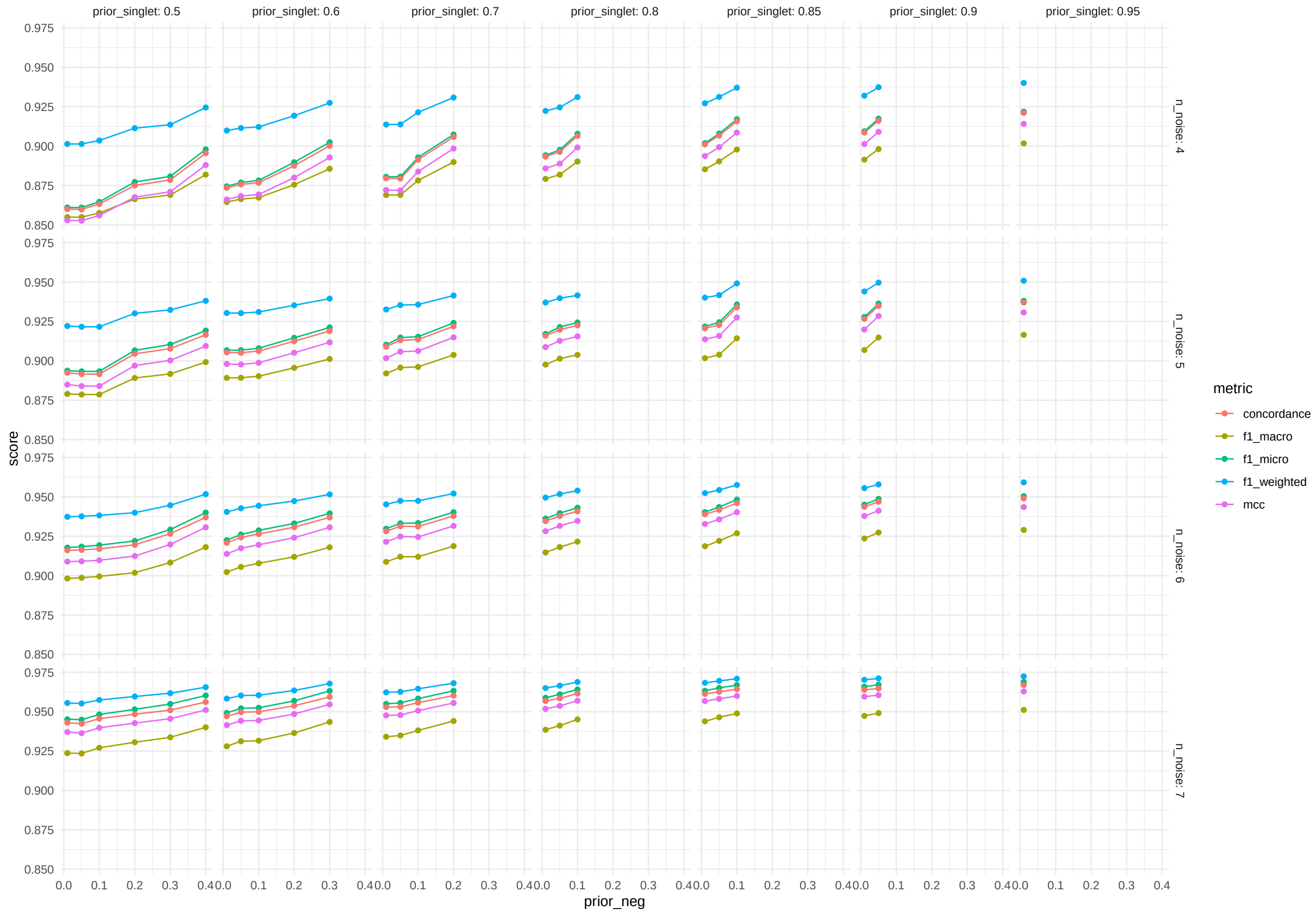
HashSolo – all metrics vs prior_neg – mcginnis_ms
