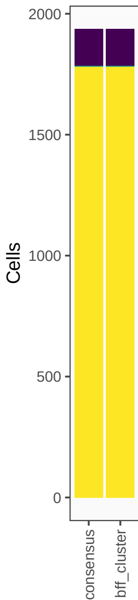
Consensus
