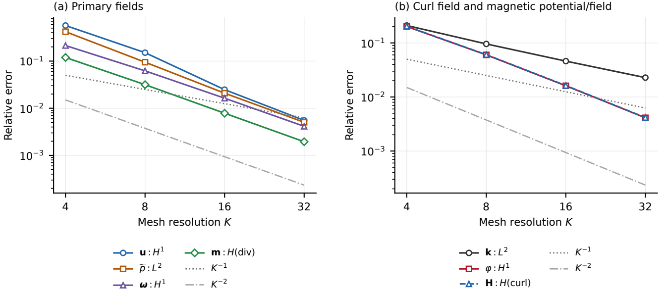
Figure 3: Relative errors for the second-order discretization using the same manufactured solution and \Delta t = 1/K . (a) Velocity, averaged modified pressure, angular velocity, and magnetization. (b) Auxiliary curl field, magnetic potential, and magnetic field. The horizontal coordinate is K = 4, 8, 16, 32 , increasing from left to right. Reference lines proportional to K^{-1} and K^{-2} distinguish the nearly quadratic decay of the principal errors from the approximately first-order L^2 decay for \mathbf{k} .
